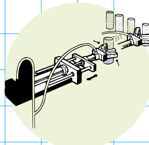
Air Cylinder/Chuck Driver
